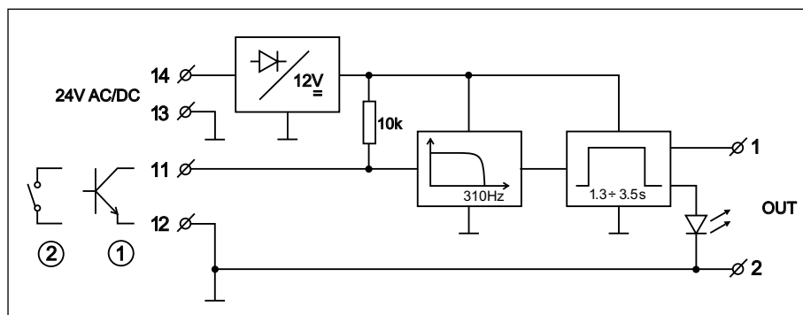
Fig.3 Connections of the UWI.
