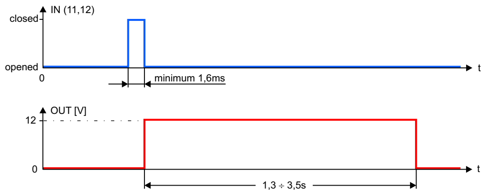
Fig.2 Regulation method and timing diagram.
